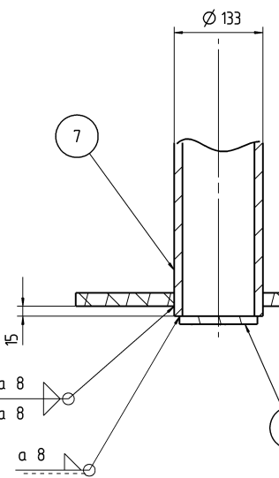
SECTION E-E SCALE 1:5
